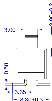
SCHEMATIC(SHORTING)
