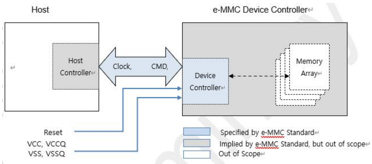
Figure 2 - e-MMC System Overview
