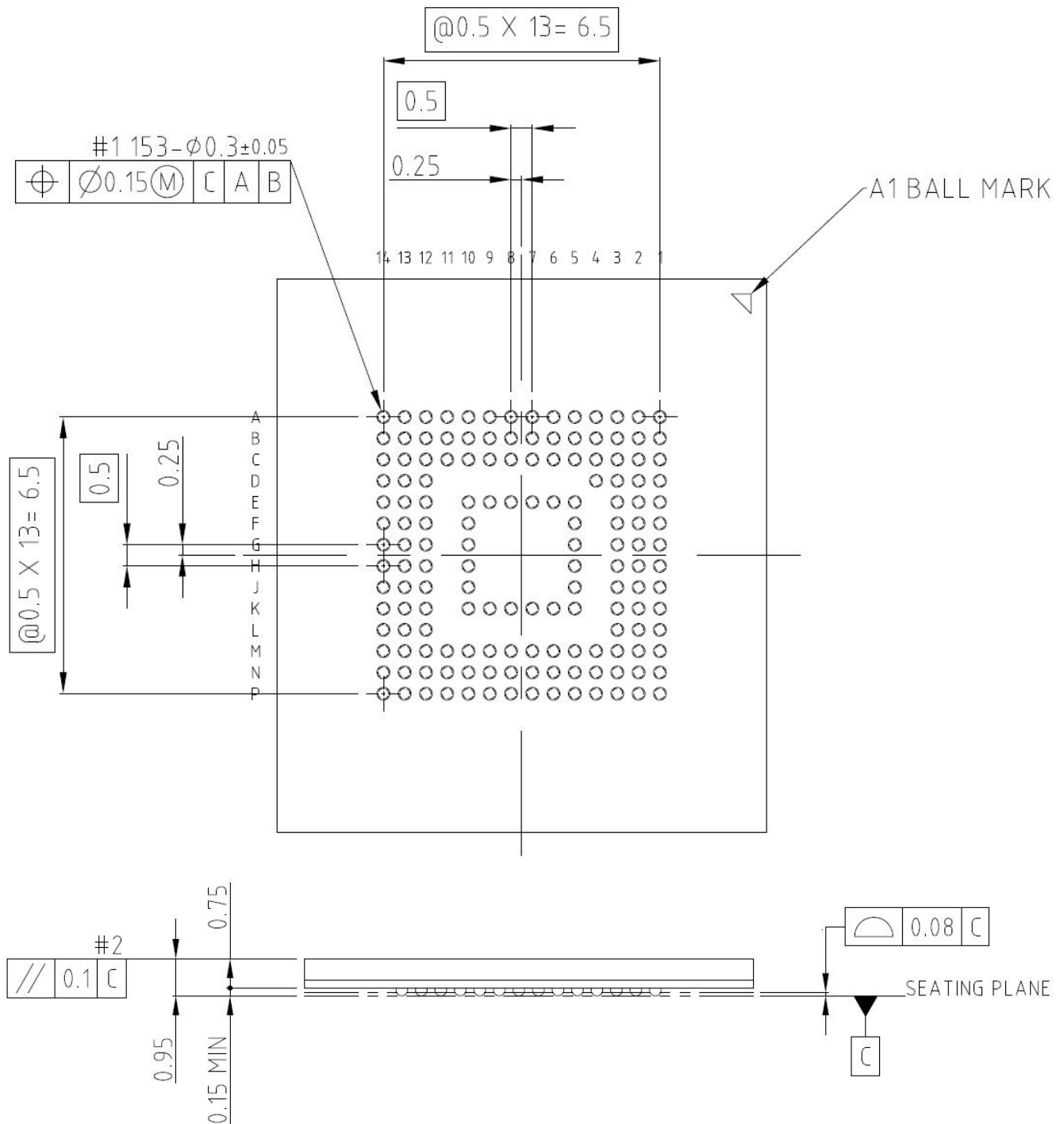
Figure 5 – 11.5 x 13.0 x 1.0mm Bottom &amp; side View
