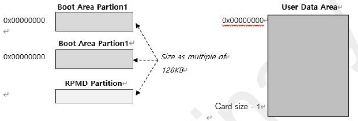
Figure 3 - e-MMC memory organization at time zero
