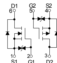
Dual N-Channel MOSFET
