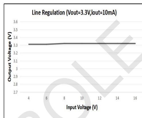
Figure 4. Line Regulation
