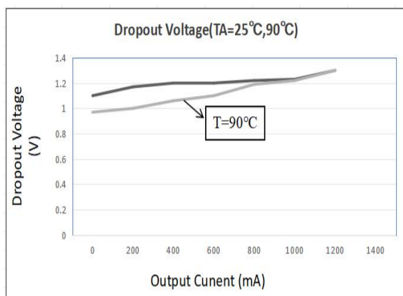
Figure 3. Dropout Voltage
