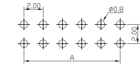
RECOMMEND P. C. B LAYOUT PCB TOLERANCE: \pm 0.05 (TOP VIEW)
