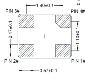
[底部视图]
