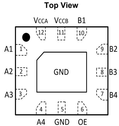
Fig.5-2. GT0104: SC (QFN2.0×2.0-12L) Package
