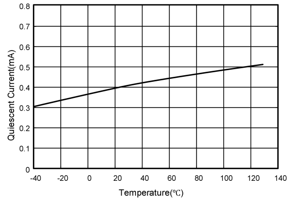
Fig.7-2. Quiescent Current vs Temperature
