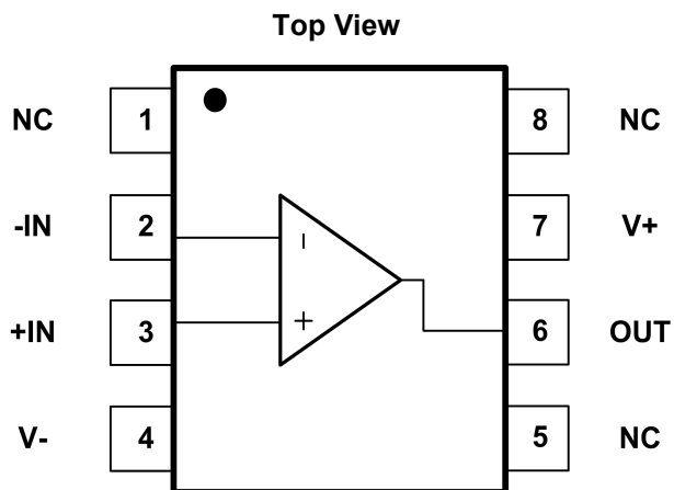
Fig.4-2. GT8531: P8(SOP8) Package
