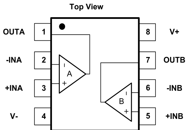
Fig.4-3. GT8532: P8(SOP8) Package GT8532: M8(MSOP8) Package
