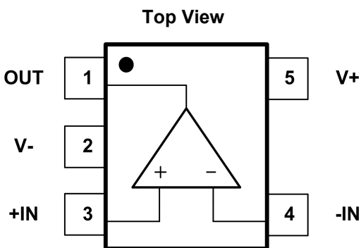
Fig.4-1. GT8531: S5(SOT23-5) Package
