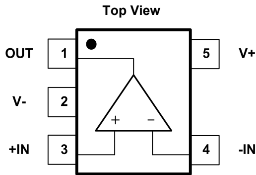
Fig.4-1. GT8561: S5(SOT23-5) Package
