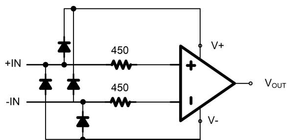
Fig.9-1. Equivalent Input Circuit
