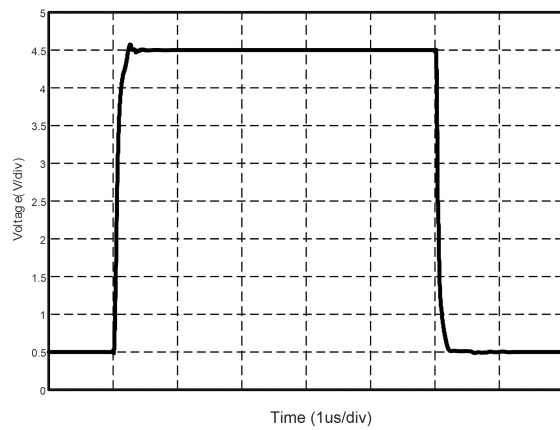
Fig.7-3. Large-Signal Step Response
