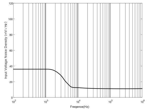
Fig.7-6. Input Voltage Noise Density vs Frequency
