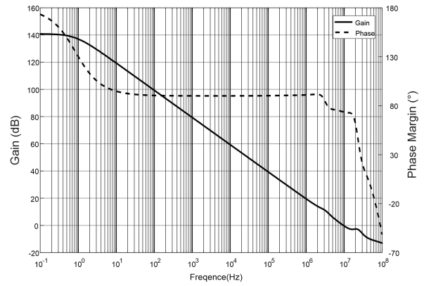
Fig.7-2. Open-Loop Gain and Phase vs Frequency
