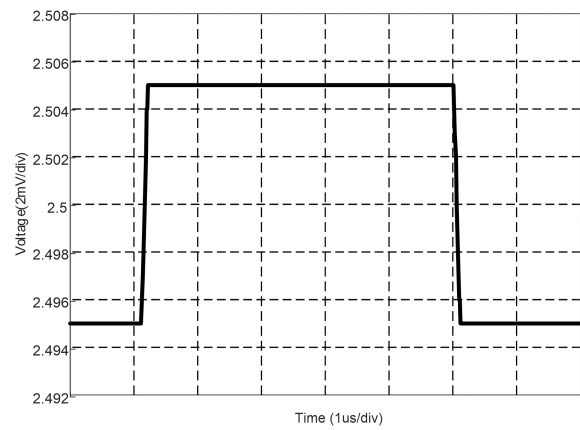
Fig.7-4. Small-Signal Step Response
