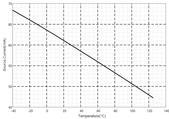
Fig.7-5. Source Current vs Temperature
