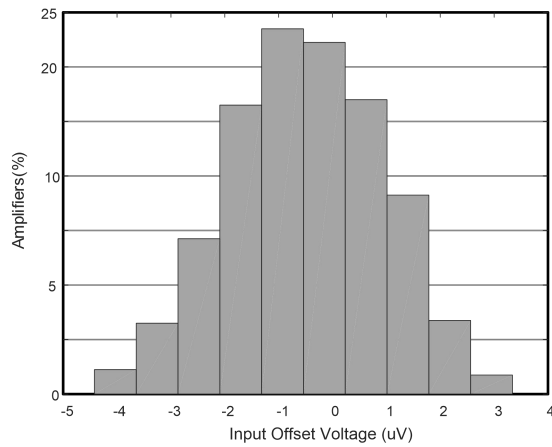
Fig.7-1. Offset Voltage Distribution
