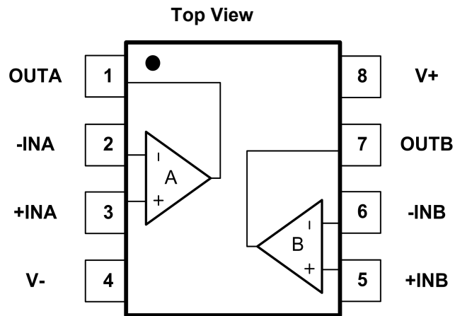
Fig.4-3. GT8562: P8(SOP8) Package GT8562: M8(MSOP8) Package
