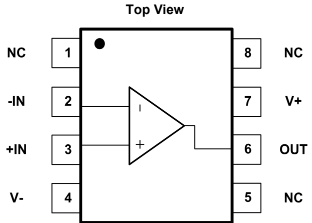
Fig.4-2. GT8561: P8(SOP8) Package
