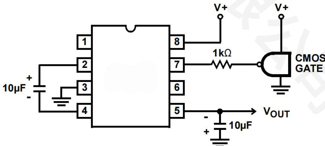
FIGURE 16. EXTERNAL CLOCKING
