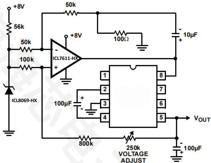
FIGURE 21. REGULATING THE OUTPU VOLTAGE
