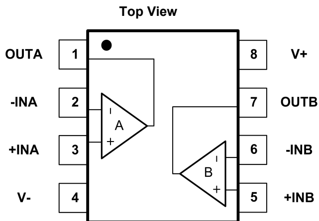
Fig.4-3. GT8552: P8(SOP8) Package GT8552: M8(MSOP8) Package
