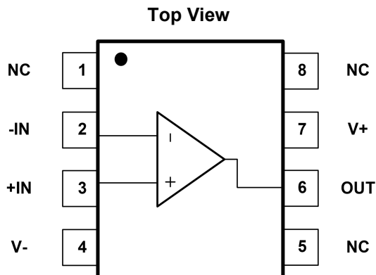
Fig.4-2. GT8551: P8(SOP8) Package GT8551: M8(MSOP8) Package
