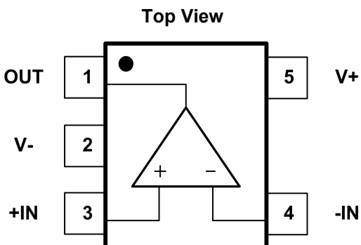
Fig.4-1. GT8551: S5(SOT23-5) Package
