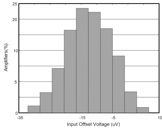
Fig.7-1. Offset Voltage Distribution
