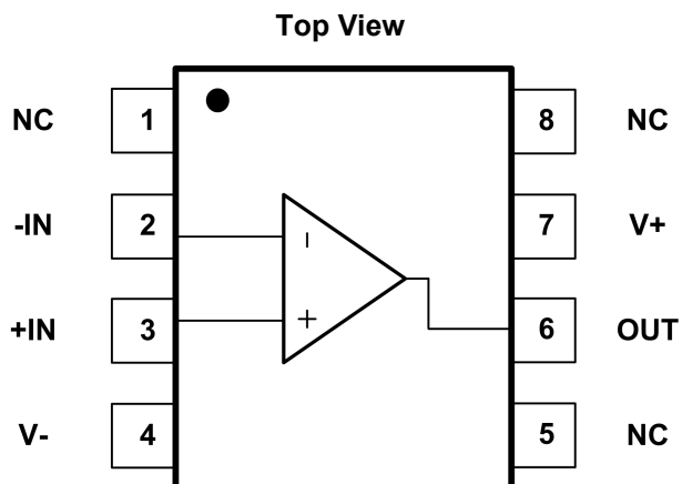
Fig.4-2. GT8501: P8(SOP8) Package
