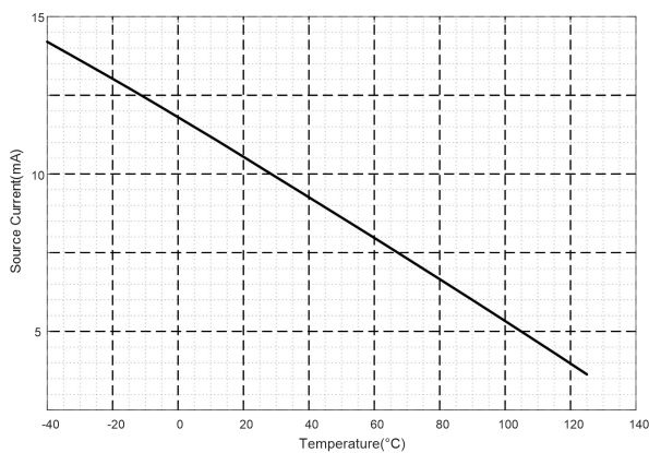
Fig.7-5. Source Current vs Temperature
