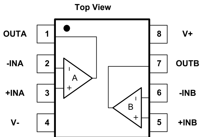
Fig.4-3. GT8502: P8(SOP8) Package GT8502: M8(MSOP8) Package
