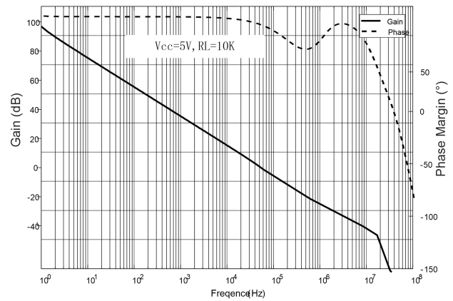
Fig.7-2. Open-Loop Gain and Phase vs Frequency
