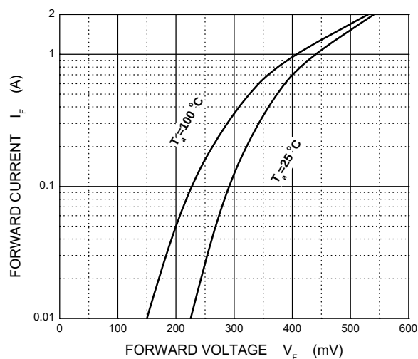
FIG.2-TYPICAL FORWARD CHARACTERISTICS
