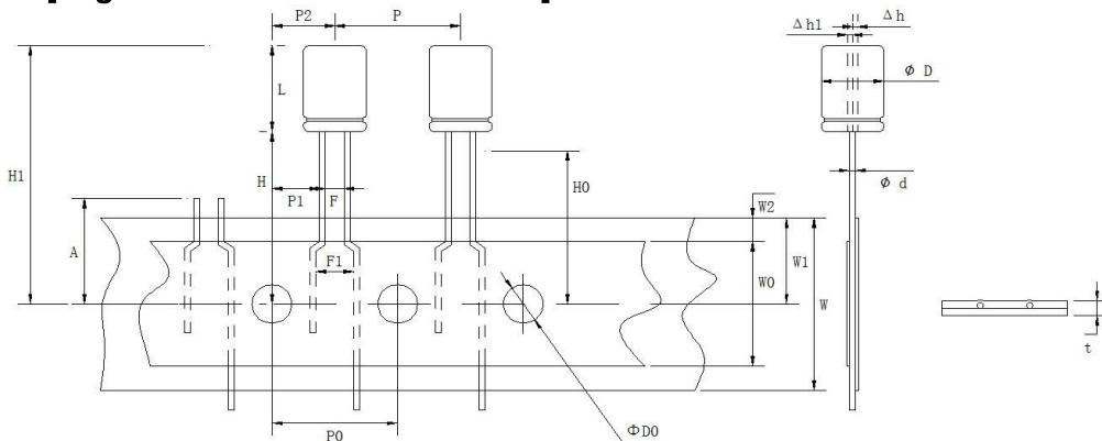
[ Fig. 3 (Diameter for \Phi 5.5 to \Phi 8 ) ]
