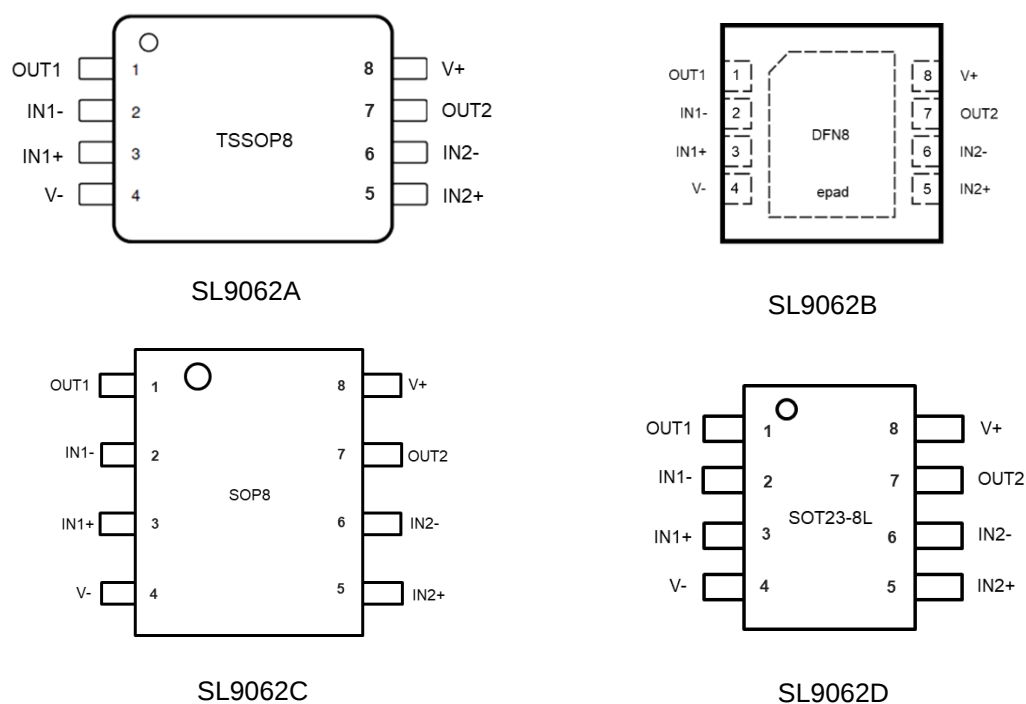
Figure 3 SL9062A/B/C/D Pinouts
