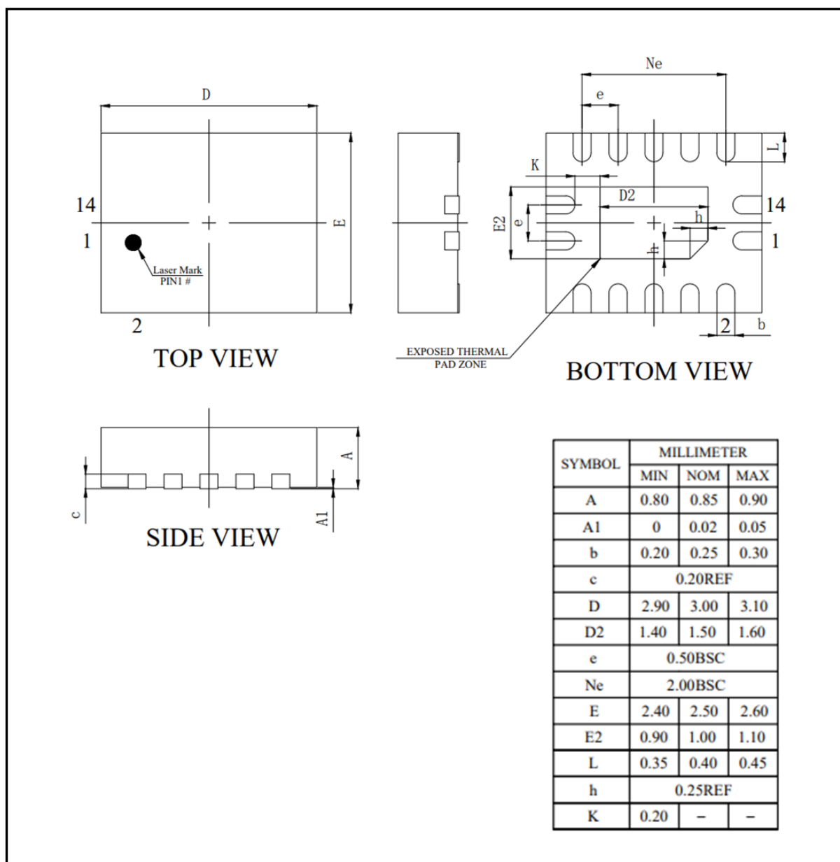
Figure 21 QFN14 Mechanical Data and Package Dimensions
