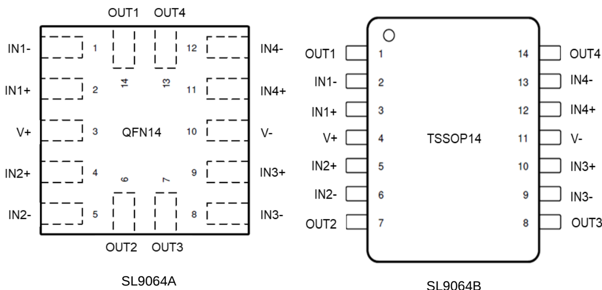
Figure 5 SL9064A/B Pinouts
