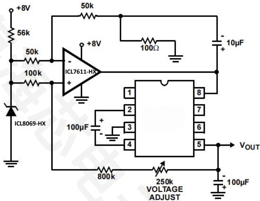
FIGURE 21. REGULATING THE OUTPU VOLTAGE
