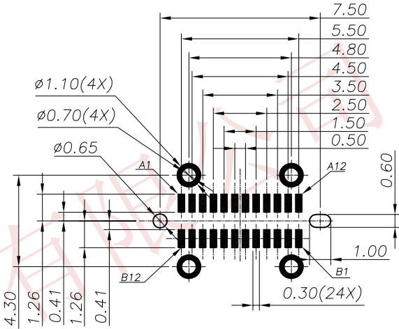
RECOMMENDED PCB LAYOUT(TOP VIEW) THICKNESS 1.0±0.1MM;DEFAULT TOLERANCE:±0.05
