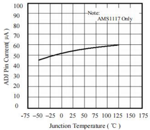
ADJ Pin Current VS. Temperature
