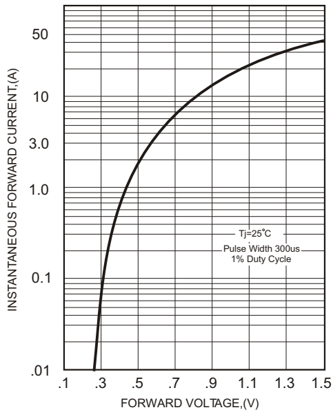
FIG.2-TYPICAL FORWARD
