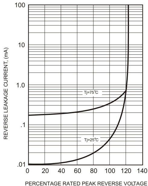
FIG.5 - TYPICAL REVERSE
