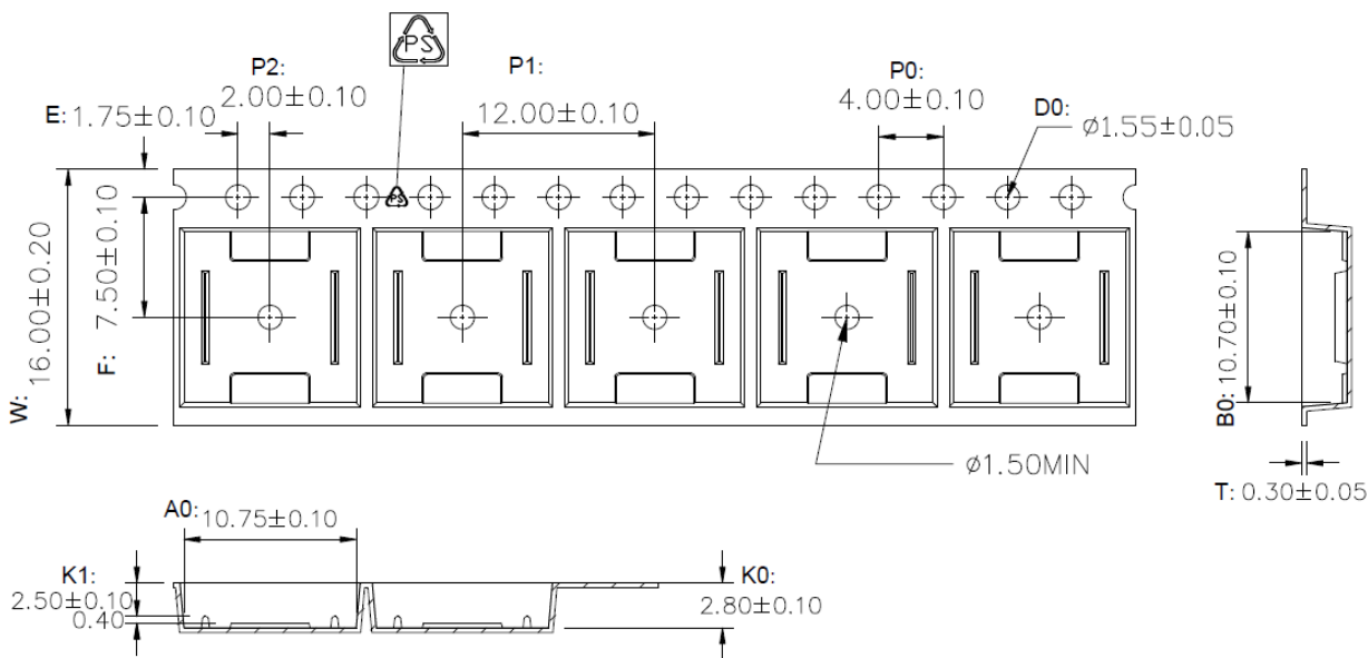
Figure 12.1 Tape Information
