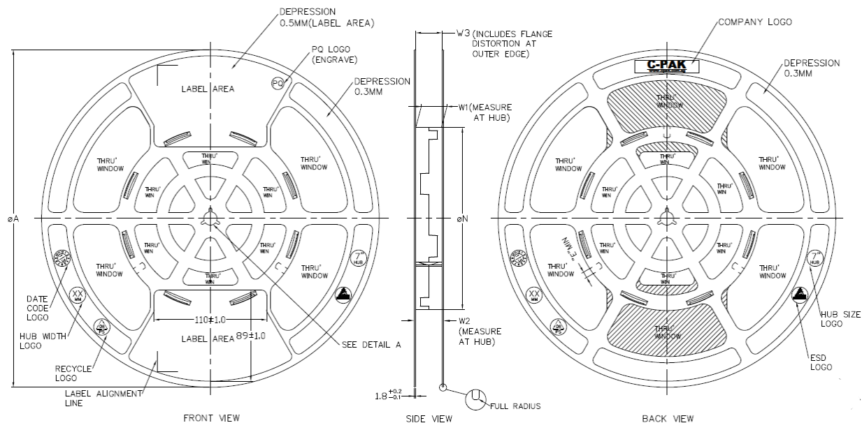
Figure 12.1 Tape Information
