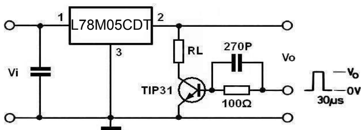
Load Regulation
