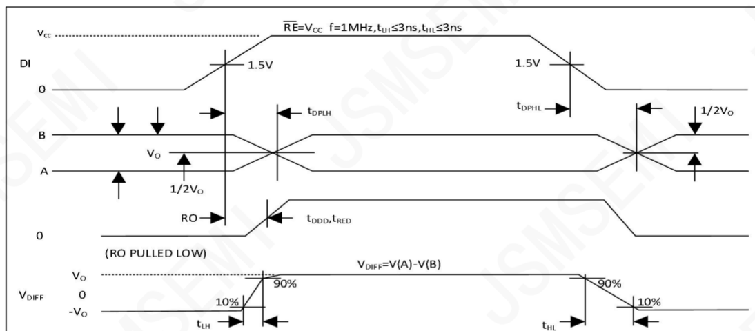
Figure 3. Driver Propagation Delays
