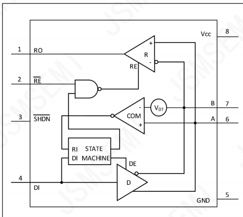
MAX13487/MAX13488 Block Diagram
