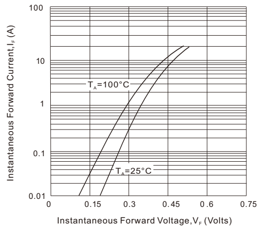
FIG.2-TYPICAL FORWARD CHARACTERISTICS
