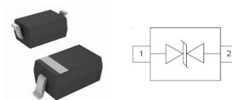
SOD-323
