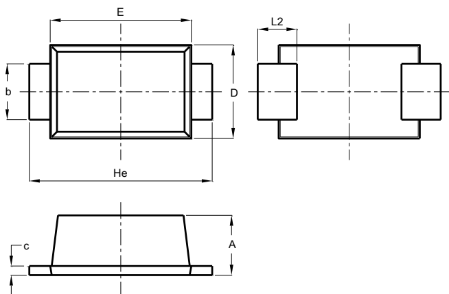
SOD123FL
