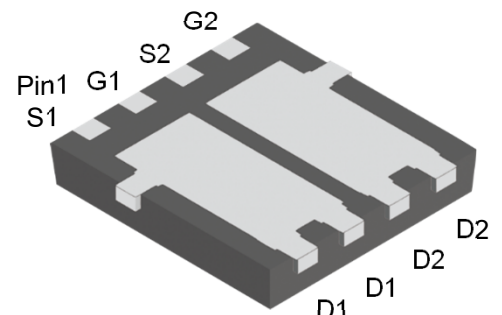
PDFN3333-8L (Bottom View)
