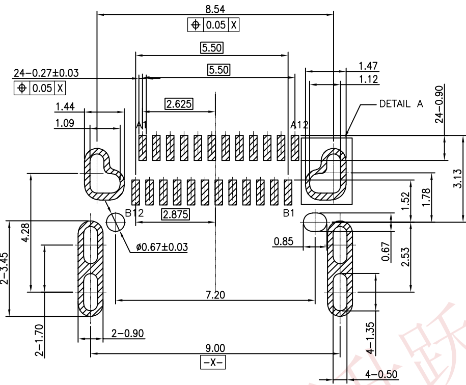
SCALE 2:1 RECOMMENDED PCB LAYOUT(TOP VIEW) Thickness 1.0mm (TOLERANCE=±0.05mm)
