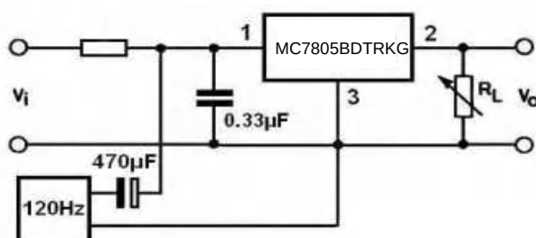
Ripple Rejection
