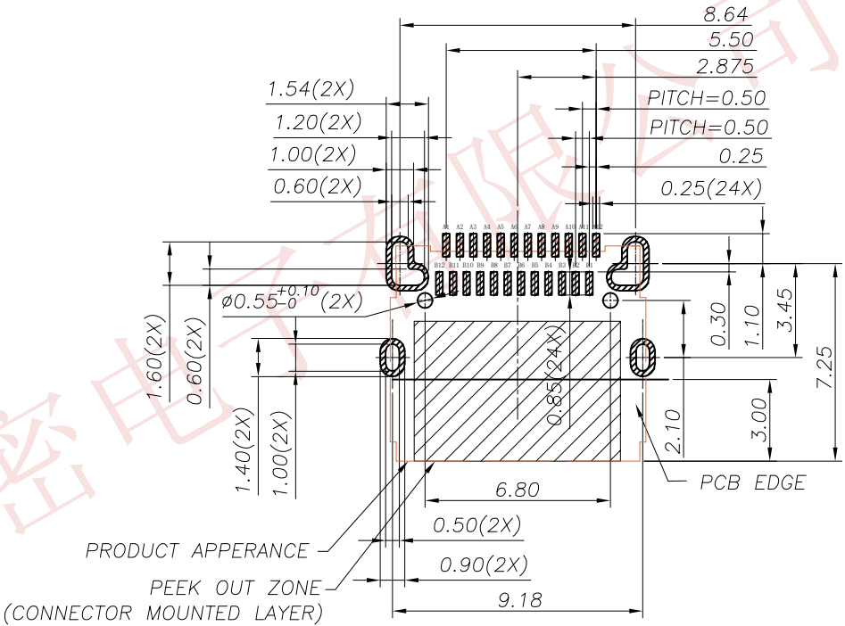
RECOMMENDED PCB LAYOUT(TOP VIEW) THICKNESS 1.6 MM;DEFAULT TOLERANCE:±0.05
