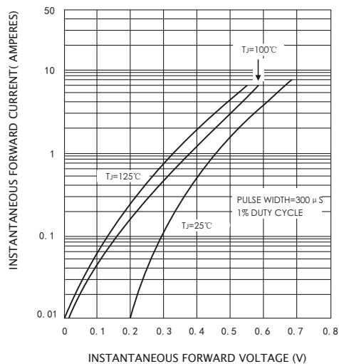
FIG.2-TYPICAL FORWARD CHARACTERISTICS
