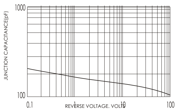
FIG.5-TYPICAL JUNCTION CAPACITANCE
