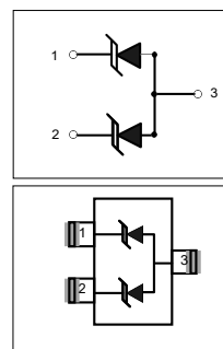
Schematic & PIN Configuration
