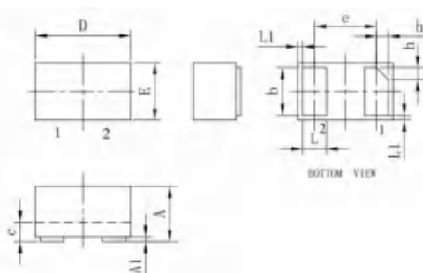
DFN1006-2L
