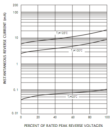
FIG.4-TYPICAL REVERSE CHARACTERISTICS
