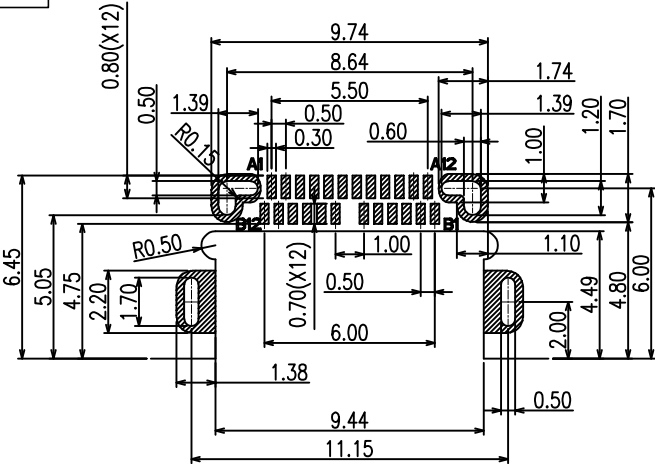
RECOMMENDED P.C.B. LAYOUT (THICKNESS:0.80MM) TOLERANCE UNSPECIFIED ±0.05mm
