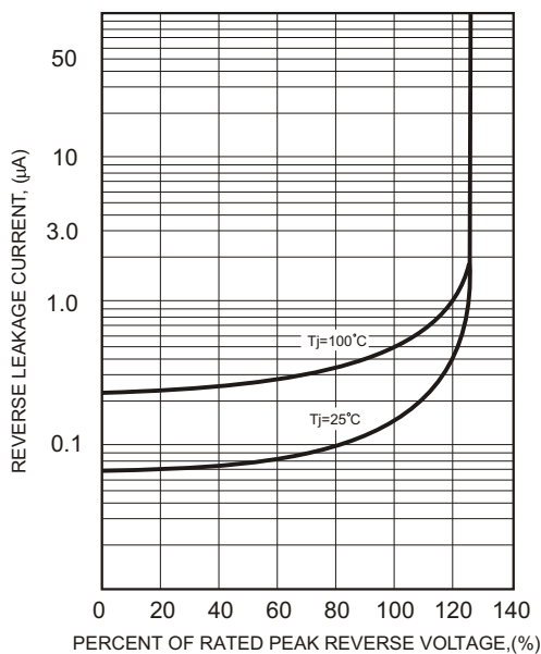
FIG.3-TYPICAL REVERSE CHARACTERISTICS
