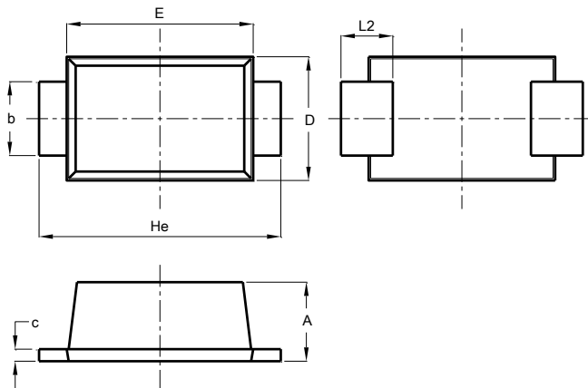
SOD123FL
