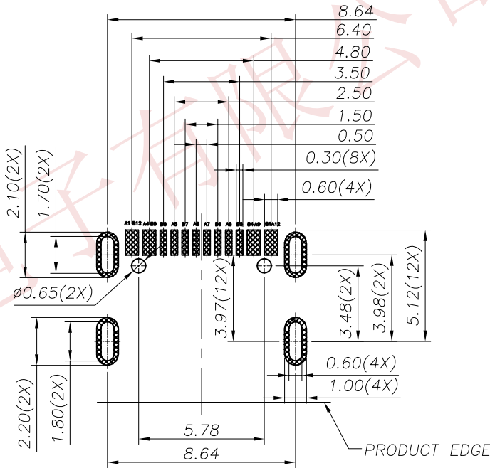
RECOMMENDED PCB LAYOUT(TOP VIEW) THICKNESS 2.00MM;DEFAULT TOLERANCE:±0.05
