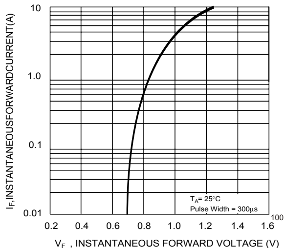
FIG.2-TYPICAL FORWARD CHARACTERISTICS
