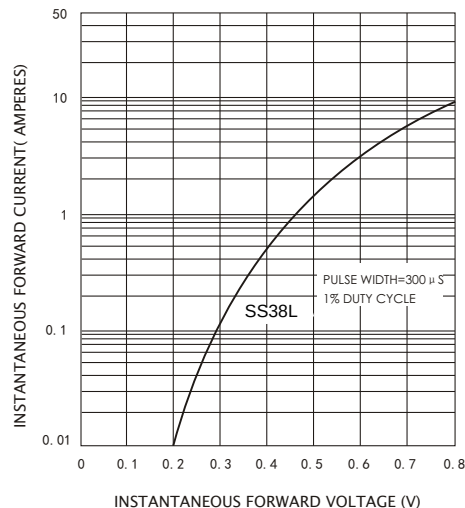
FIG.2-TYPICAL FORWARD CHARACTERISTICS
