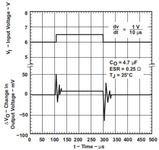
Figure 14. HG76350 Line Transient Response
