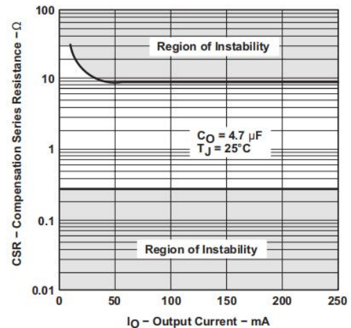
Figure 16. Compensation Series Resistance (CSR) vs Output Current
