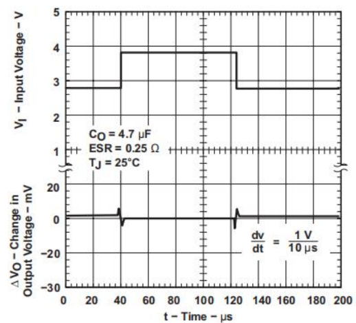
Figure 12. HG76318 Line Transient Response
