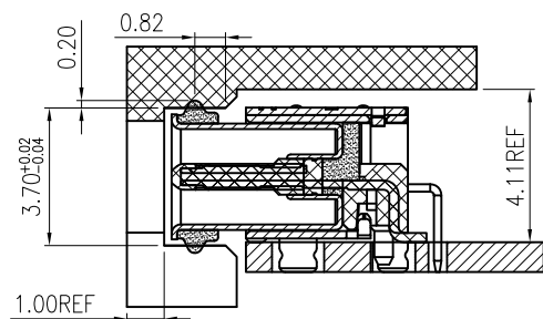
RECOMMENDED OPENING DIMENSIONS OF CASE MATING AREA WITH SEALING RING SECTION:A-A
