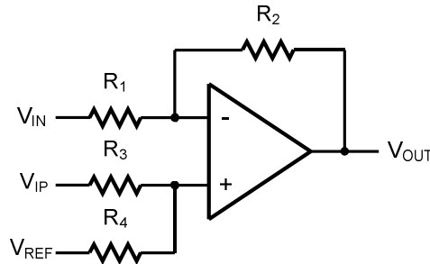
Figure 4. Differential Amplifier
