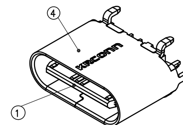
CAP ASSEMBLY AND MOUTING CONDITION(REF.)
