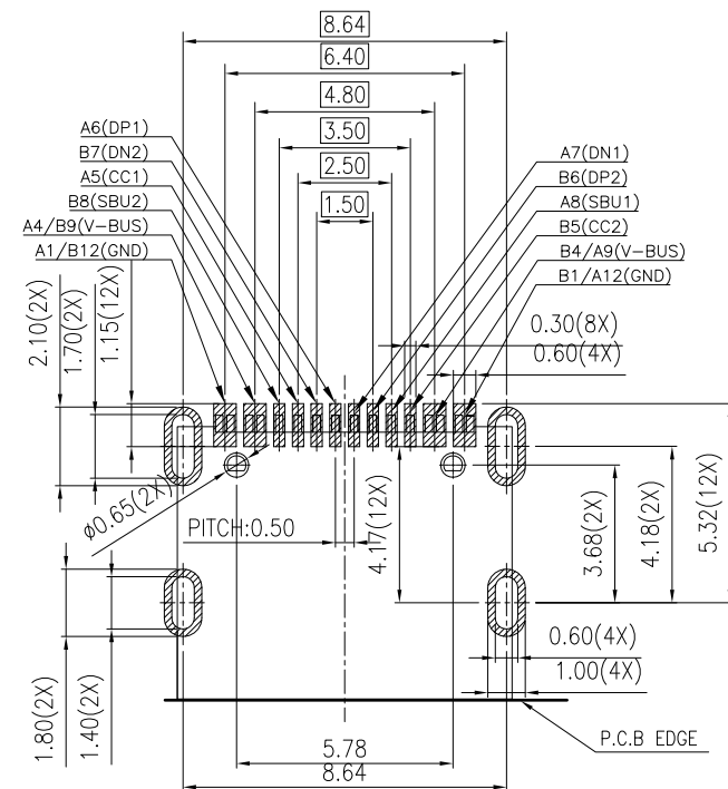
RECOMMENDED P.C.B LAYOUT (COMPONENT SIDE)
