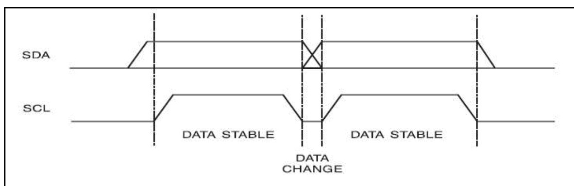
Figure 1. Data Validity
