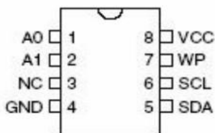
DIP-8/SOP-8/MSOP-8
