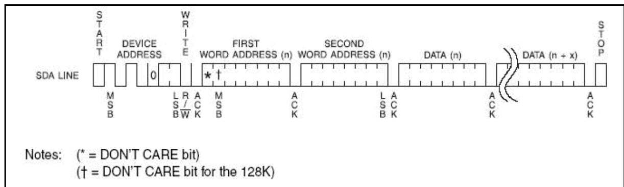
Figure 6. Page Write
