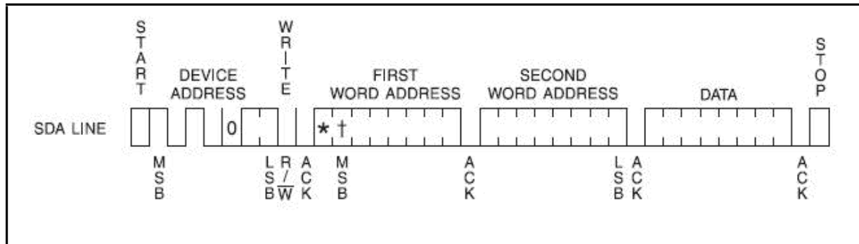
Figure 5. Byte Write
