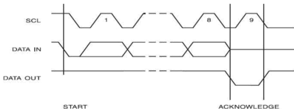
Figure 3. Output Acknowledge
