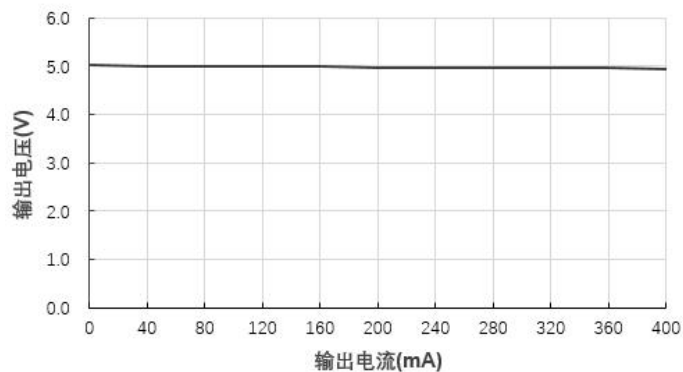
输出电压 VS 输出电流 IB1205S-2W@ (Vin=12V)
