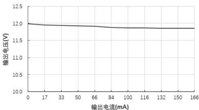
输出电压 VS 输出电流 IB1212S-2W@ (Vin=12V)
