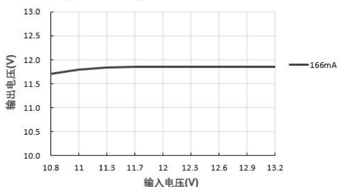
输出电压 VS 输入电压 (IB1212S-2WR3)
