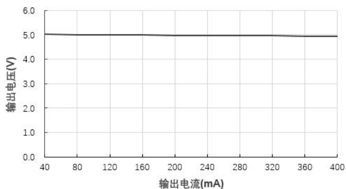
输出电压 VS 输出电流 IB2405S-2W@ (Vin=24V)
