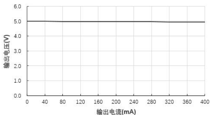
输出电压 VS 输出电流 IB0505S-2W@ (Vin=5V)
