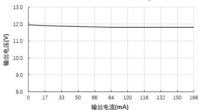
输出电压 VS 输出电流 IB0512S-2W@ (Vin=5V)
