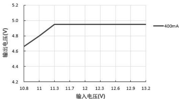
输出电压 VS 输入电压 (IB1205S-2WR3)
