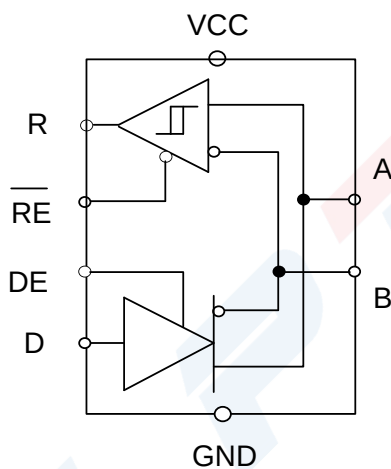
Figure 9-1. MAX3485ESA-Y Block Diagram
