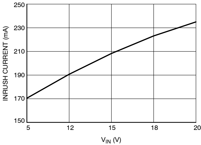
Figure 7. Inrush Current vs. V IN for C LOAD = 1000 μF @ 25°C
